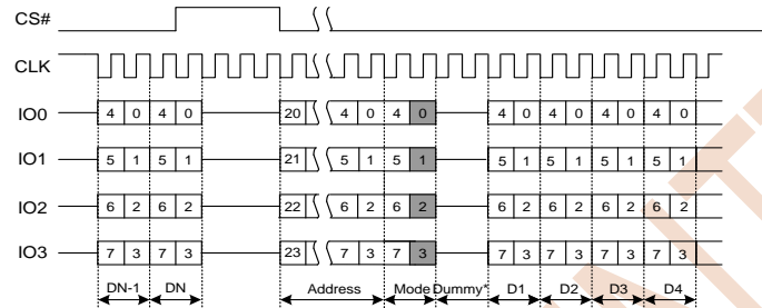
Figure 7.22 Word Read Quad I/O Instruction(Initial command or previous M5-4 =10)
