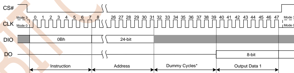
Figure 7.14a Fast Read Instruction
