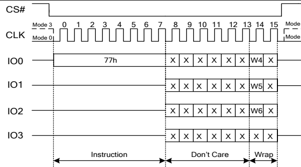
Figure 7.25 Set Burst with Wrap Instruction
