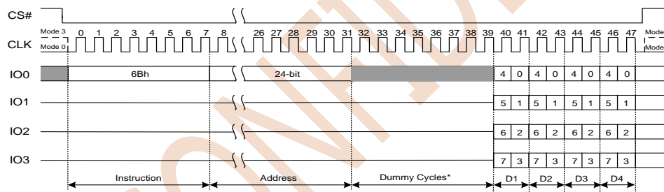
Figure 7.16 Fast Read Quad Output Instruction
