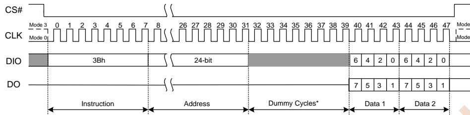
Figure 7.15 Fast Read Dual Output Instruction Sequence Diagram
