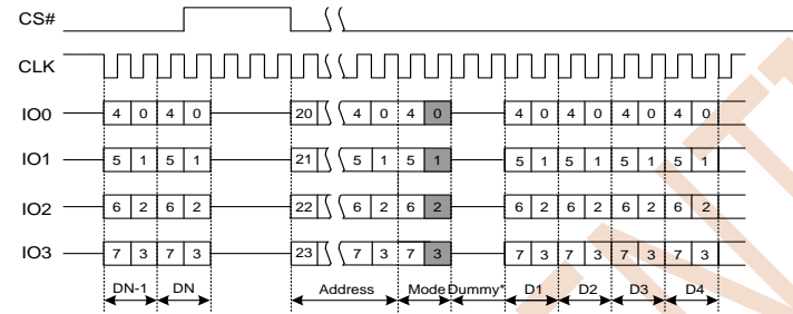
Figure 7.22 Word Read Quad I/O Instruction(Initial command or previous M5-4 =10)
