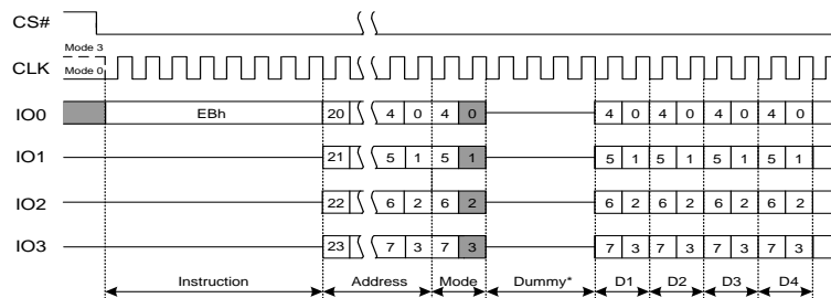
Figure 7.19a Fast Read Quad I/O Instruction(Initial command or previous M5-4 ≠10)
