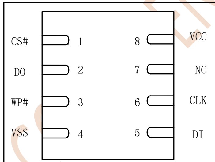
Figure 3.2 DFN8
