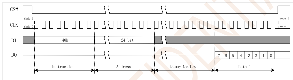
Figure 7.35 Read Security Registers Instruction
