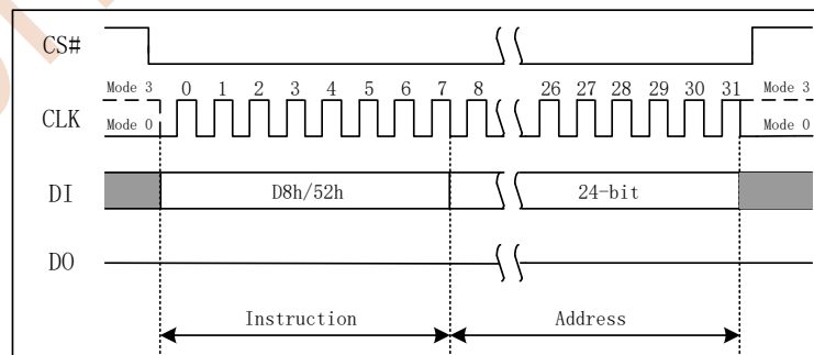
Figure 7.7 Block Erase Instruction
