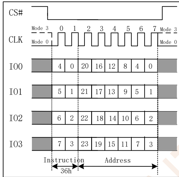
Figure 7.34b Individual Block/Sector Lock Instruction (QPI Mode)
