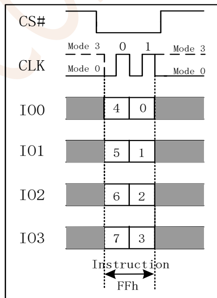
Figure 7.46 Exit QPI Instruction (QPI Mode only)
