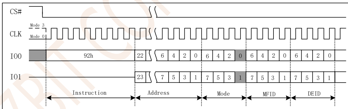
Figure 7.39 Read Manufacturer/Device ID Dual I/O Instruction
