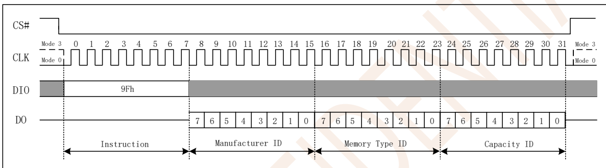
Figure 7.29a Read JEDEC ID(SPI Mode)
