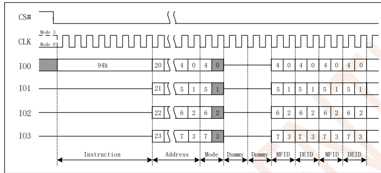
Figure 7.40 Read Manufacturer/Device ID Quad I/O Instruction
