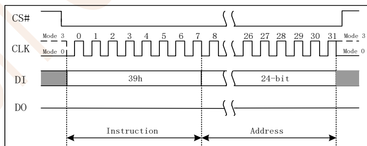
Figure 7.35a Individual Block/Sector Unlock Instruction (SPI Mode)
