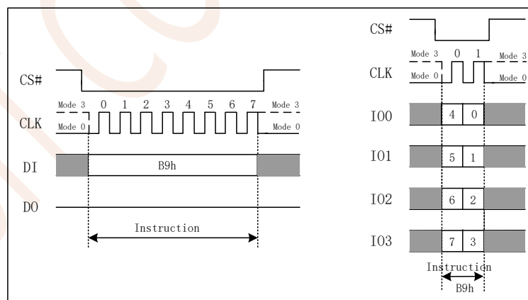
Figure 7.25 Deep Power-down Instruction(SPI and QPI Mode)
