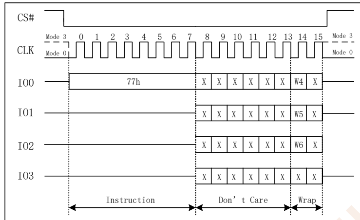
Figure 7.23 Set Burst with Wrap Instruction
