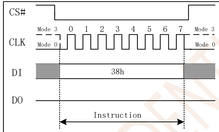
Figure 7.45 Enter QPI Instruction (SPI Mode only)
