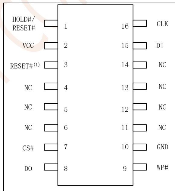
Figure 3.3 SOP16
