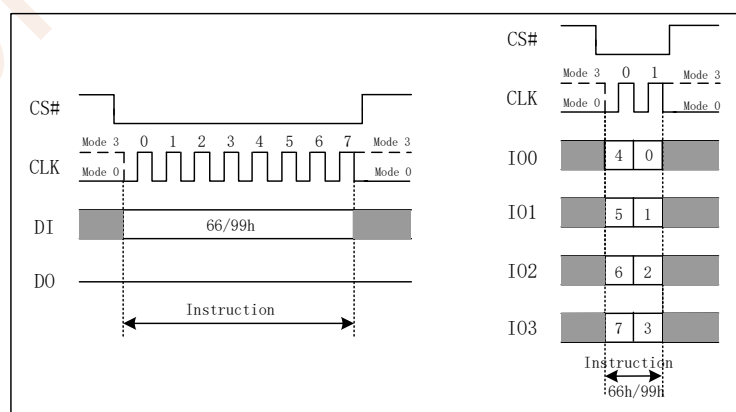
Figure 7.24 Software Reset Instruction (SPI and QPI Mode)
