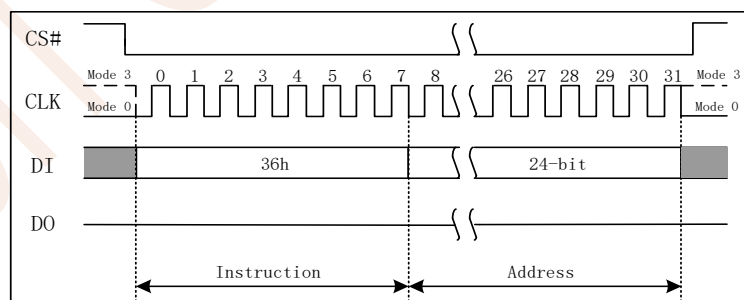
Figure 7.34a Individual Block/Sector Lock Instruction(SPI Mode)
