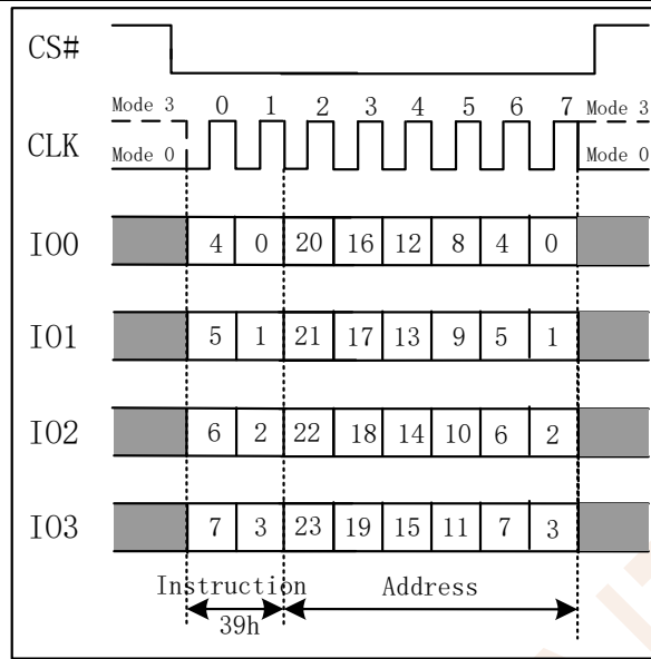
Figure 7.35b Individual Block/Sector Unlock Instruction(QPI Mode)
