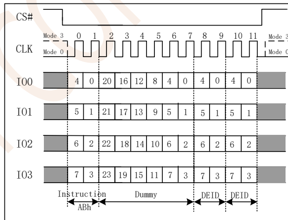
Figure 6.28b Release Power-down / Device ID (QPI Mode)
