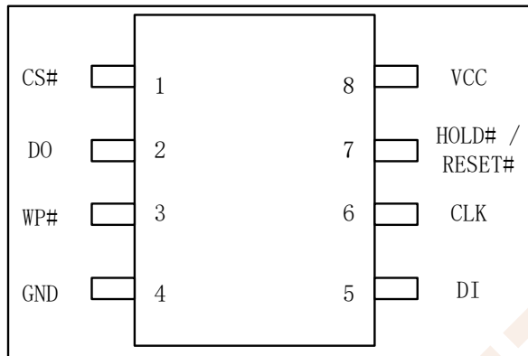
Figure 3.1 SOP8
