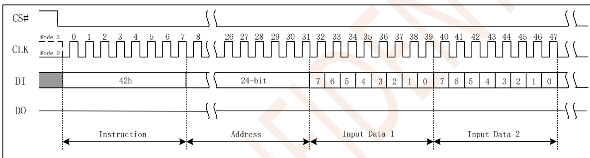
Figure 7.33 Program Security Registers Instruction
