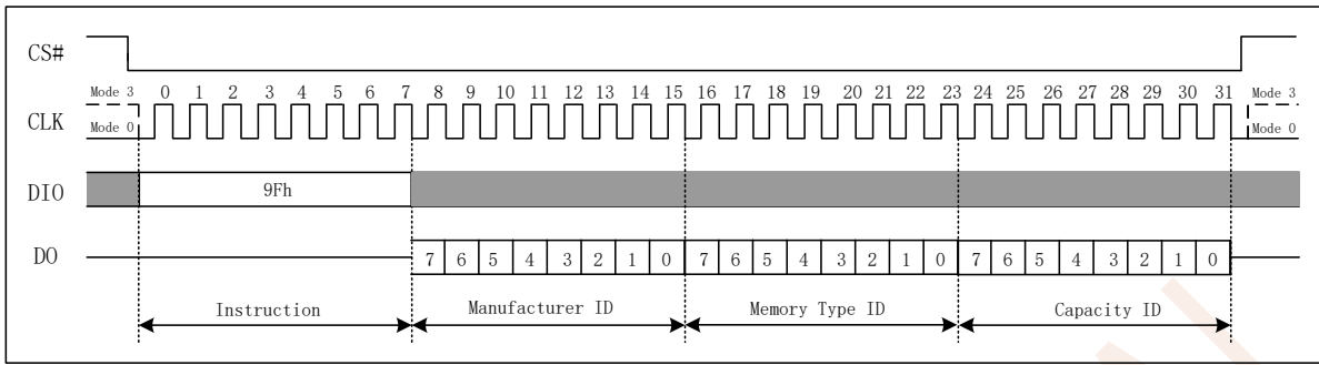
Figure 7.30a Read JEDEC ID (SPI Mode)
