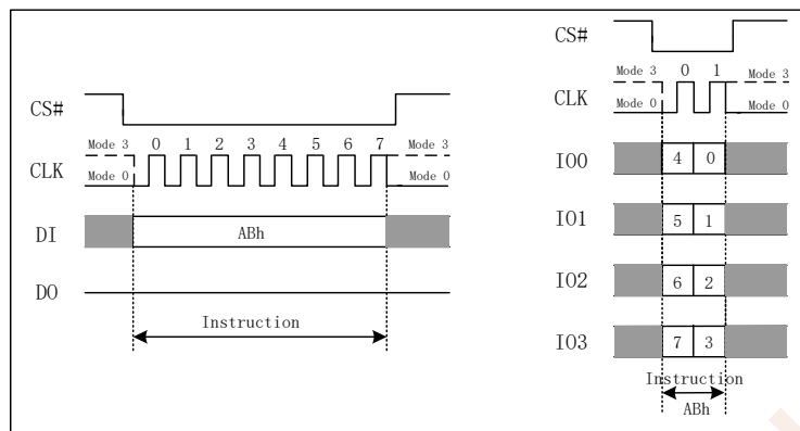
Figure 7.27 Release Power-down Instruction (SPI and QPI Mode)
