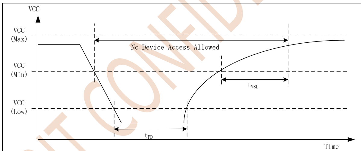
Figure 8.1 Power-up Timing
