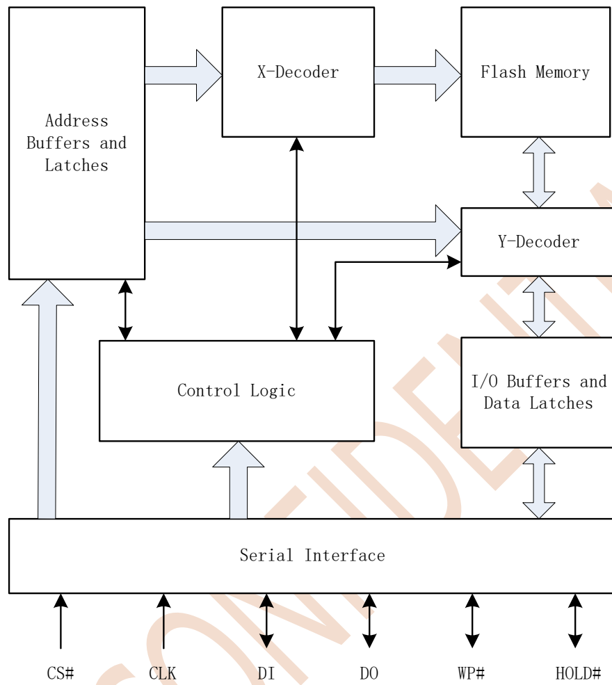
Figure 2.1 Block Diagram
