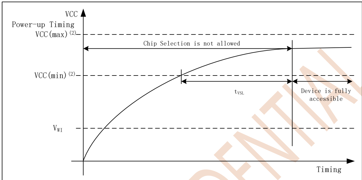
Figure 8.1 Power-up Timing
