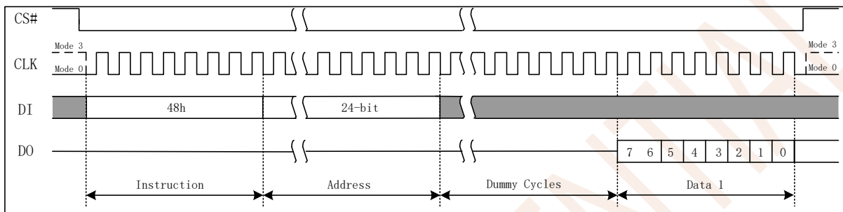
Figure 7.34 Read Security Registers Instruction
